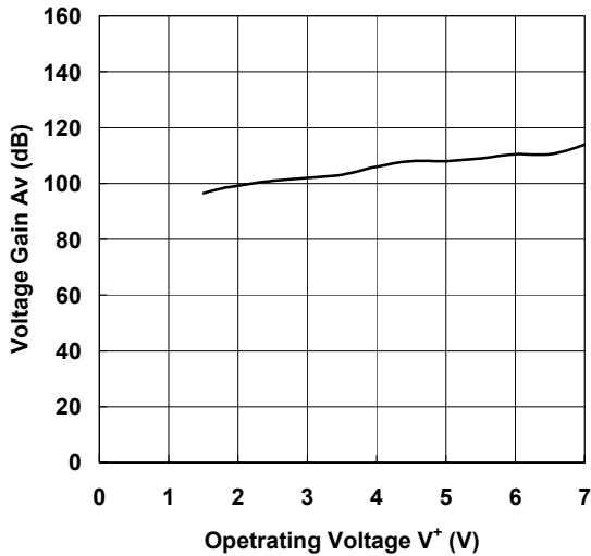
Voltage Gain vs. Operating Voltage (Ta=25°C, RL=2kΩ)
